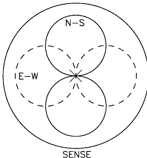
Figure 2 - Adcock DF Antenna Azimuthal Gain Patterns
