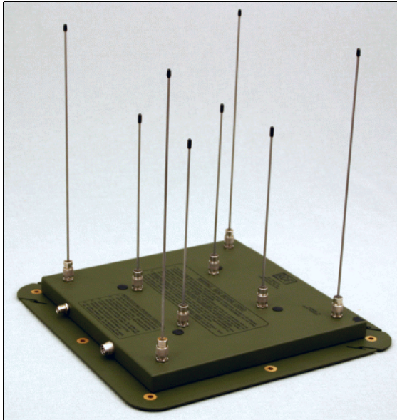
Figure 4 - DMA-1315B1 80-520 MHz Mobile Adcock DF Antenna
