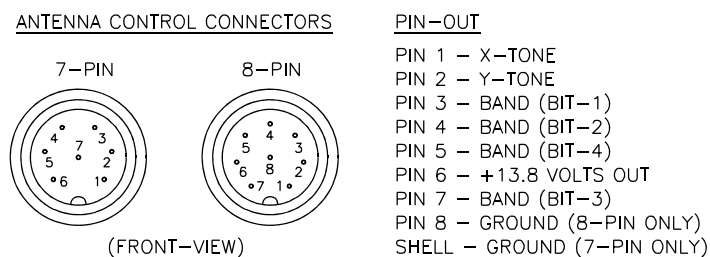
Figure 8 - Control Cable Mating Connector Pin-Outs
