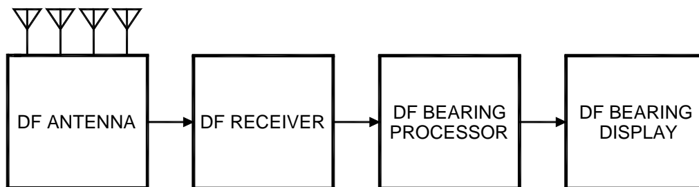
Figure 6 - Watson-Watt DF System Simplified Functional Block Diagram
