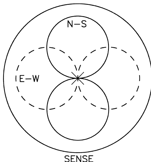
Figure 7 - Adcock DF Antenna Azimuthal Gain Patterns
