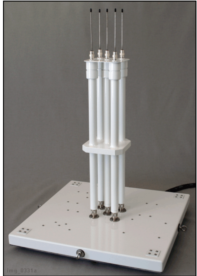
Figure 1 - DFA-1405B1 300-1,000 MHz Sleeve-Dipole Adcock DF Antenna
